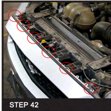
Reinstall the six 8mm bolts
