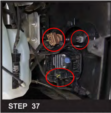
Connect the parking light, signal light, and fog light plugs for both sides
